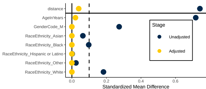
Blood Pressure
